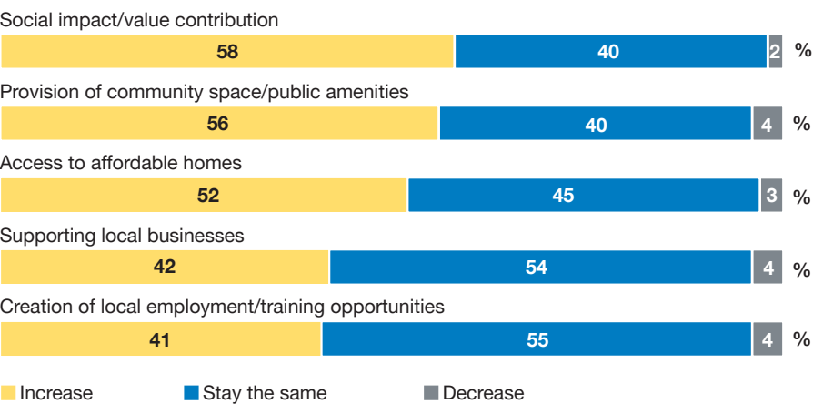
Figure 4-2 Importance of social aspects of ESG in portfolio, 2021
